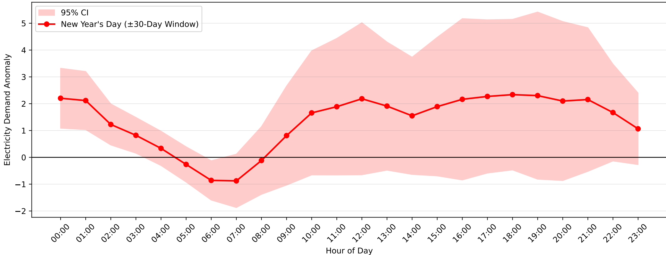
Umina Demand Anomaly: New Year's Day (2004-2017, \pm 30 -Day Window)
